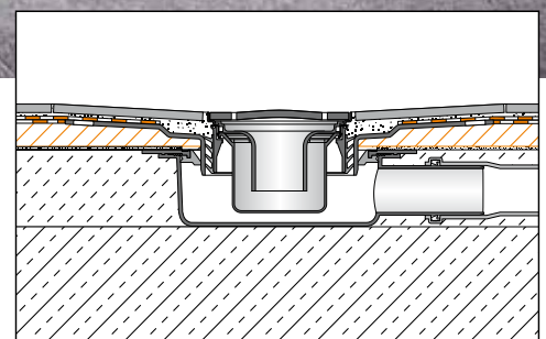
Horizontale afwatering
