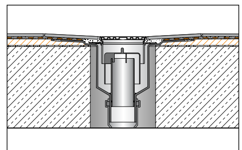
Verticale afwatering
